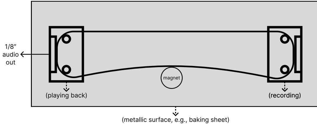
Figure 2 (bird's-eye view of the cassette players setup):
